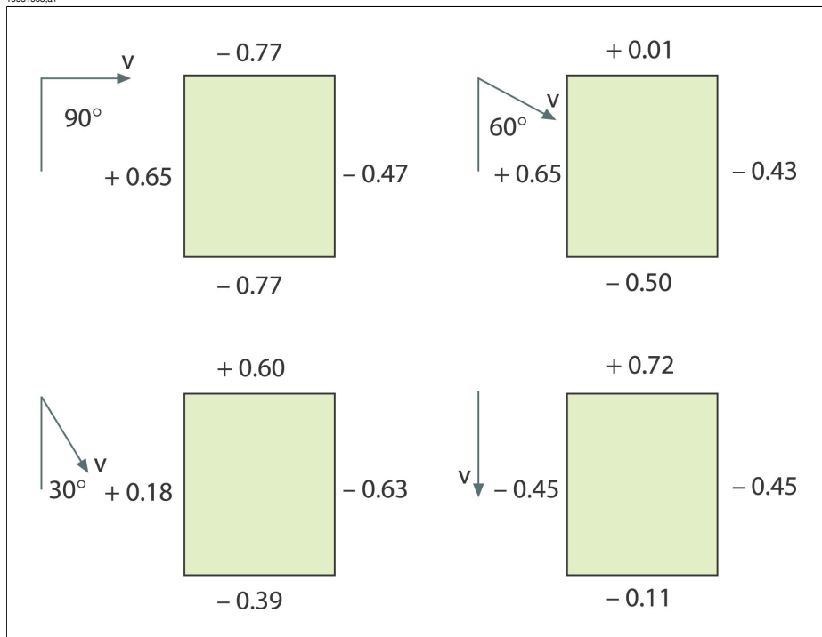
Figure 20.4 Stress concentration factor (C) distributions for various wind directions and wind velocities (v) relative to a building.
