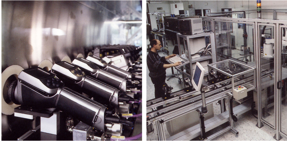
Figure 22.4 LEFT: Testing of infrared cameras in the climatic chamber; RIGHT: Robot used for camera testing and calibration
