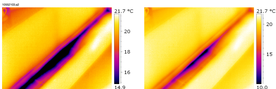
Figure 20.1 LEFT: A thermally untuned infrared image; RIGHT: A thermally tuned infrared image, after having changed level and span.
