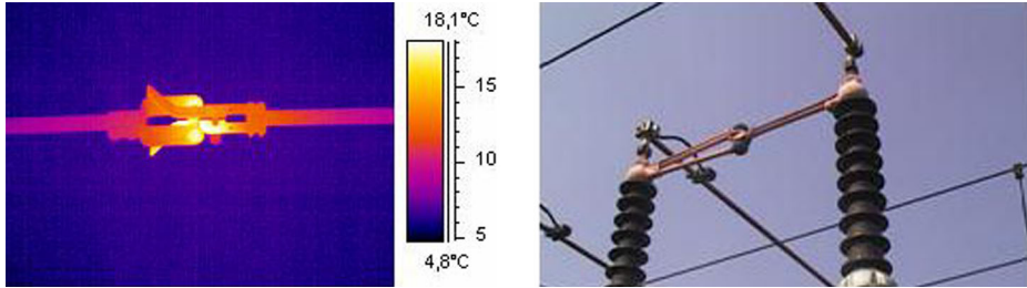
Figure 21.17 Overheating in a circuit breaker
