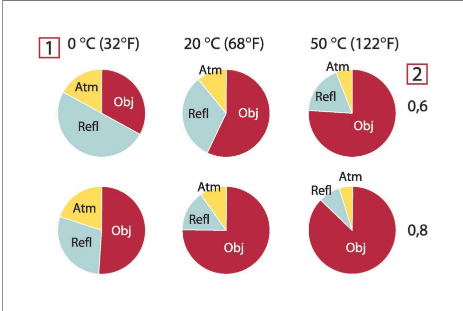
Figure 27.3 Relative magnitudes of radiation sources under varying measurement conditions (SW camera). 1: Object temperature; 2: Emittance; Obj: Object radiation; Refl: Reflected radiation; Atm: atmosphere radiation. Fixed parameters: \tau = 0.88 ; T_{\text{refl}} = 20\text{ °C} (+68 °F); T_{\text{atm}} = 20\text{ °C} (+68 °F).
