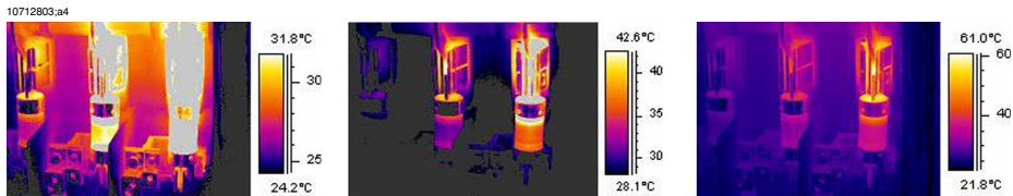
Figure 21.2 Temperature variations in a fusebox
