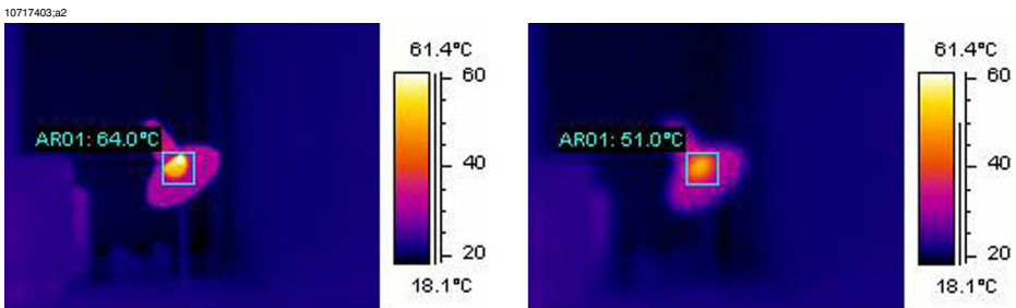
Figure 21.5 LEFT: A hot spot in focus; RIGHT: A hot spot out of focus
