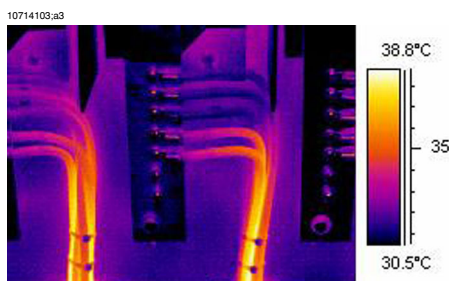
Figure 21.15 An infrared image of bundled cables
