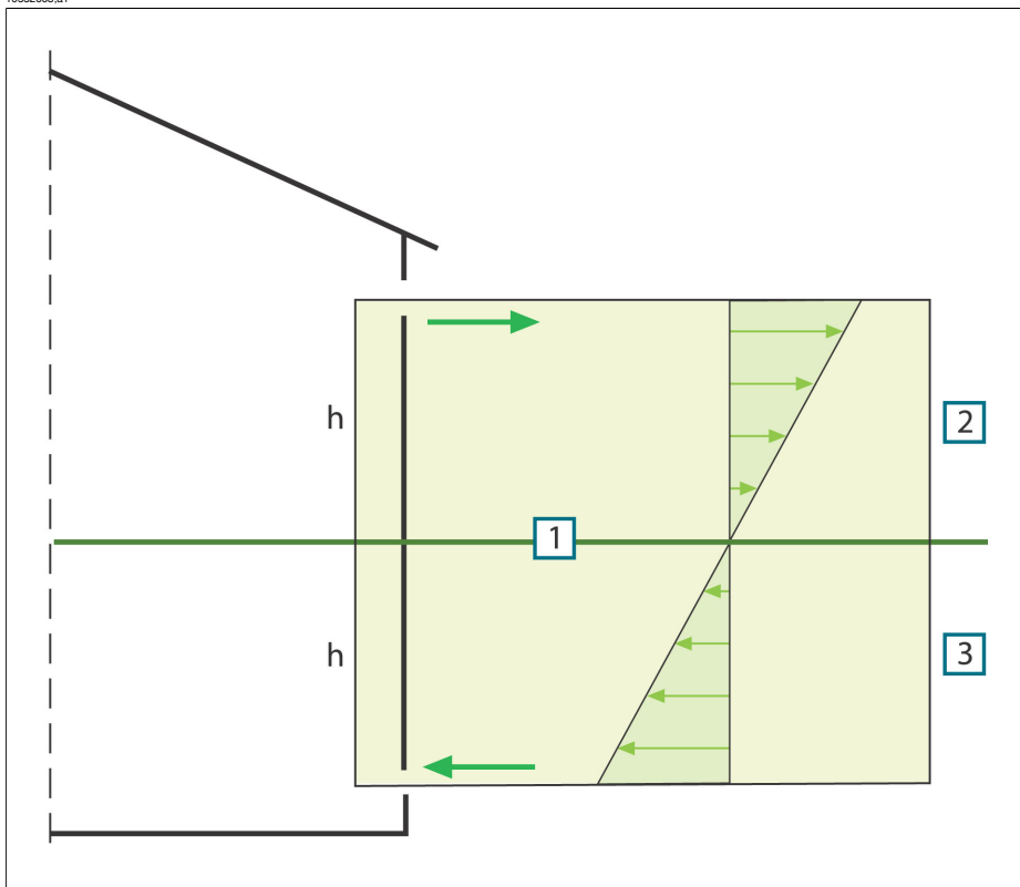
Figure 20.5 Distribution of pressures on a building with two openings and where the external temperature is lower than the internal temperature. 1: Neutral zone; 2: Positive pressure; 3: Negative pressure; h : Distance from the neutral zone in meters.
