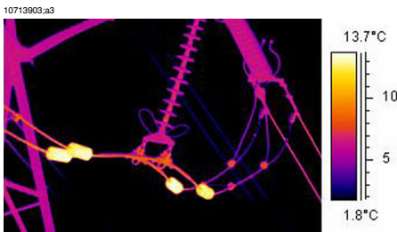
Figure 21.13 An infrared image of hot stabilizing weights
