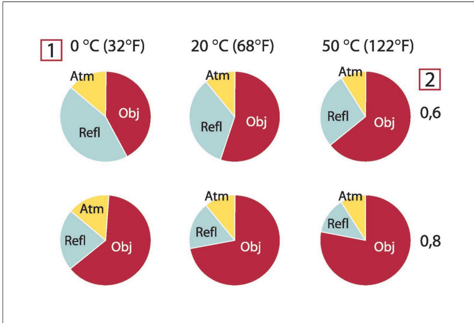
Figure 27.4 Relative magnitudes of radiation sources under varying measurement conditions (LW camera). 1 : Object temperature; 2 : Emittance; Obj : Object radiation; Refl : Reflected radiation; Atm : atmosphere radiation. Fixed parameters: \tau = 0.88 ; T_{\text{refl}} = 20 \text{ }^\circ\text{C} (+68 °F); T_{\text{atm}} = 20 \text{ }^\circ\text{C} (+68 °F).
