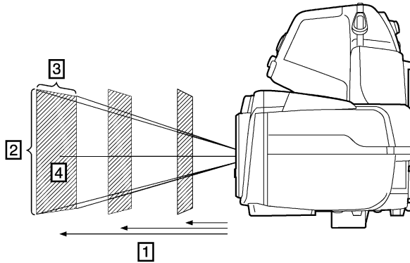
Figure 17.1 Relationship between the field of view and distance. 1: Distance to target; 2: VFOV = vertical field of view; 3: HFOV = horizontal field of view; 4: IFOV = instantaneous field of view (size of one detector element).
