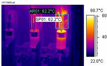
Figure 21.3 An infrared image of a fusebox where the maximum temperature is displayed
