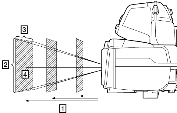
Figure 17.2 Relationship between the field of view and distance. 1: Distance to target; 2: VFOV = vertical field of view; 3: HFOV = horizontal field of view, 4: IFOV = instantaneous field of view (size of one detector element).
