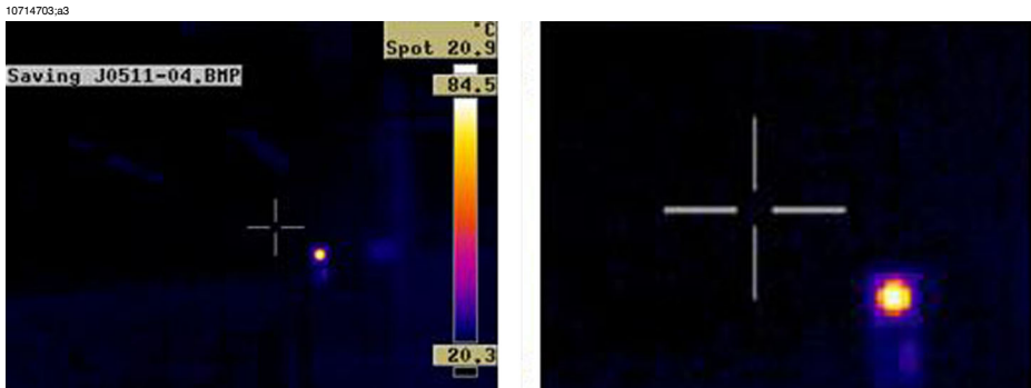
Figure 21.21 Image from the viewfinder of a ThermoCAM 695
