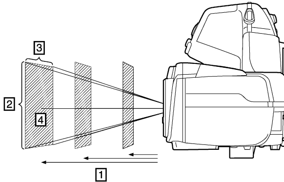
Figure 17.3 Relationship between the field of view and distance. 1: Distance to target; 2: VFOV = vertical field of view; 3: HFOV = horizontal field of view, 4: IFOV = instantaneous field of view (size of one detector element).
