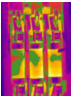
Figure 21.6 An isotherm in an infrared image of a fusebox
