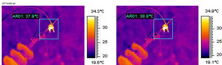
Figure 21.18 LEFT: Incorrect distance setting; RIGHT: Correct distance setting
