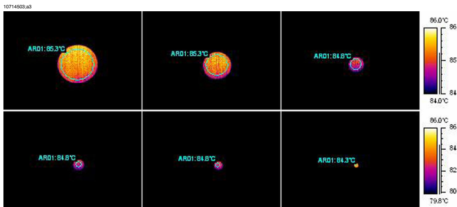
Figure 21.19 Temperature readings from a blackbody at +85°C (+185°F) at increasing distances
