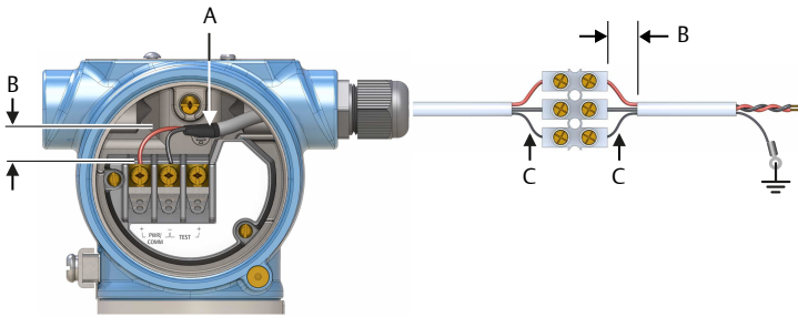
Figure 3-3: Signal Cable Shield Grounding at Power Supply End
