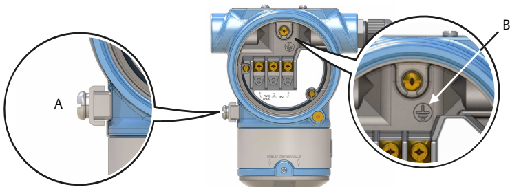
Figure 3-4: Ground Screws
