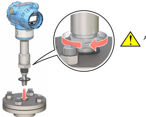
A. Tighten using the hexagon nut only
