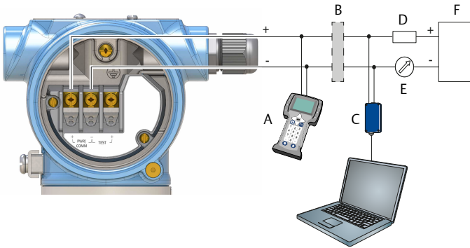
Figure 3-2: 4-20 mA/HART® Communication
