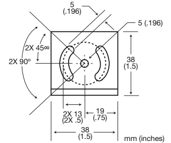
Fixed Mounting Bracket
