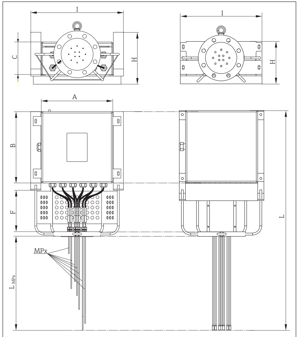
11 Design of the modular multipoint thermometer, with frame neck on the left side or with frame neck and covers on the right side. All dimensions in mm (in)
