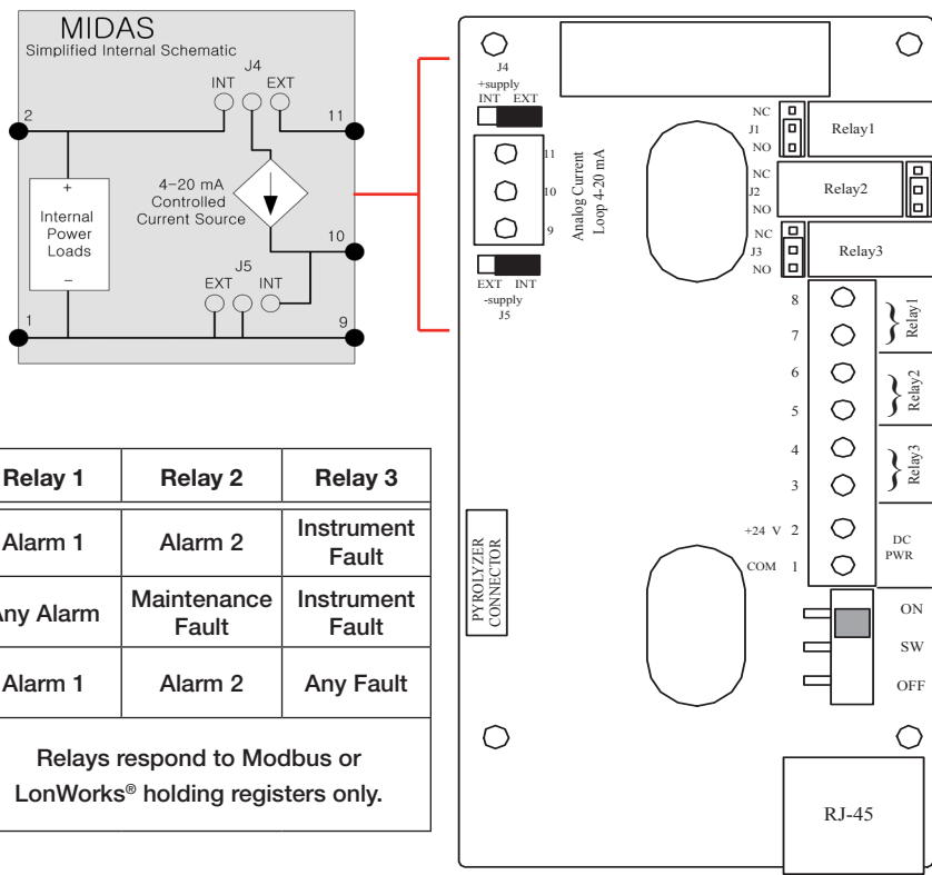
Diagram 4-6. Midas® terminal layout and identification
