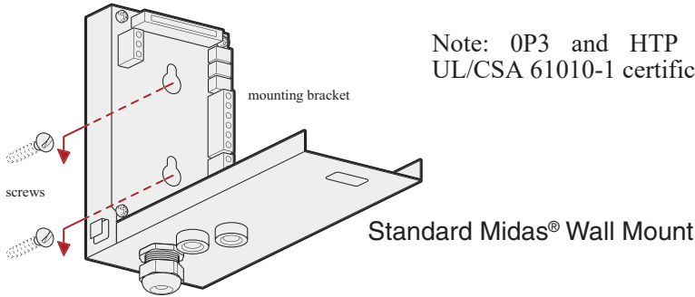
Diagram 4-3. Mechanical installation
