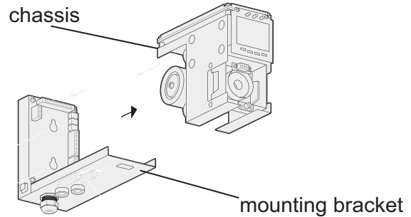
Diagram 9-5. Removing the chassis.
