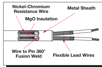
\frac{1}{2} Inch Double-Ended FIREBAR Element and Lead Configurations
