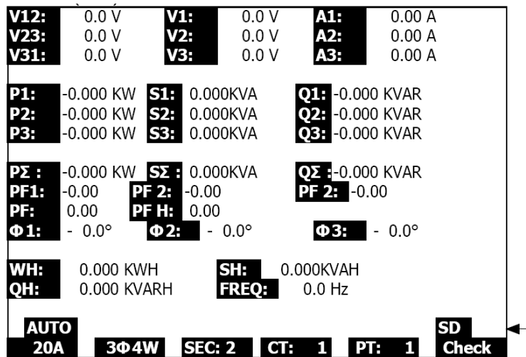
Figure 4-2: Main Screen
