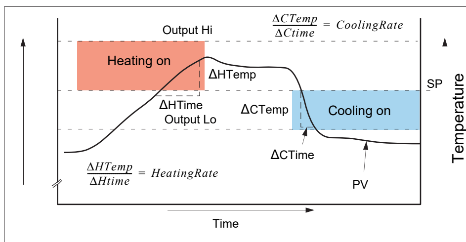
Figure 208 R2G calculation
