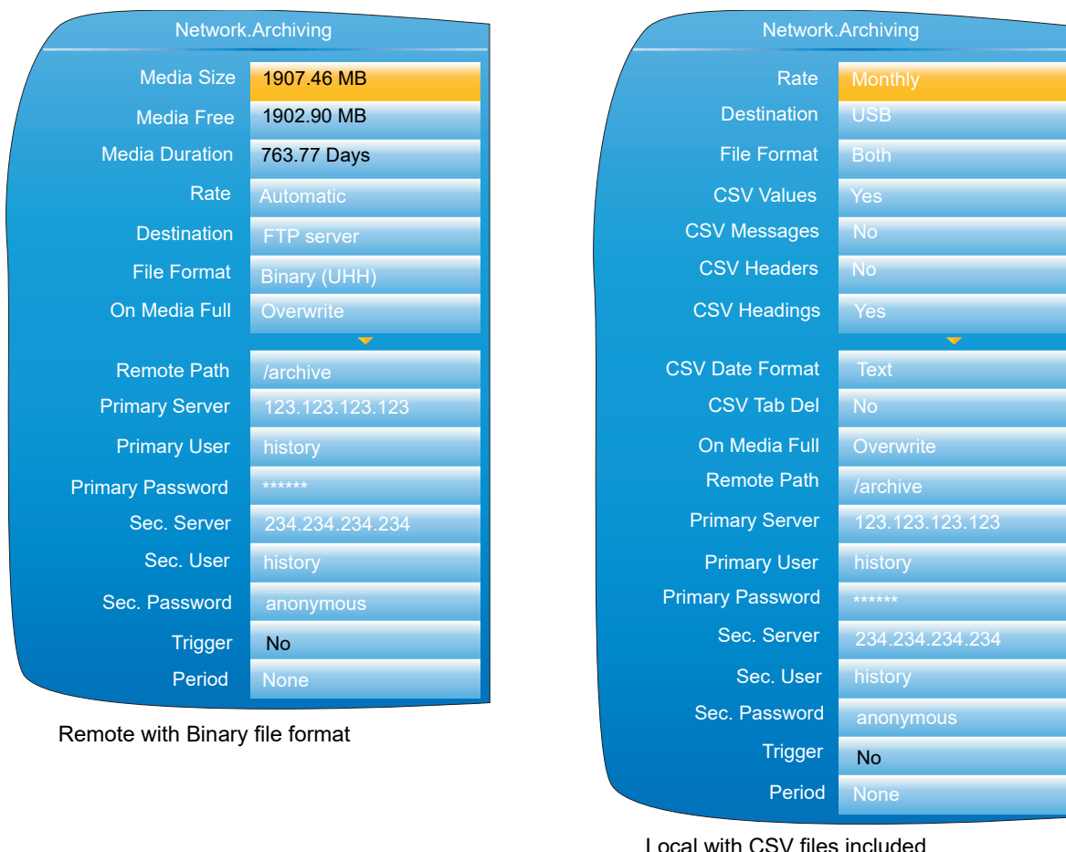
Figure 82 Unattended Archive configuration (typical settings)
