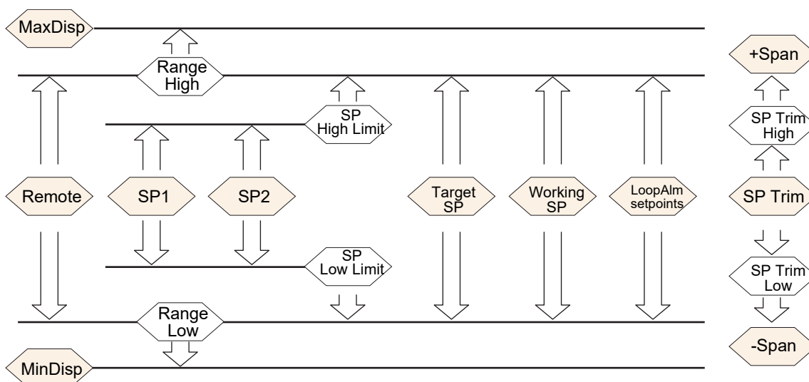
Figure 214 Setpoint Limits
