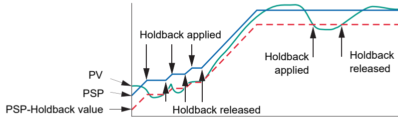
Figure 32 Holdback
