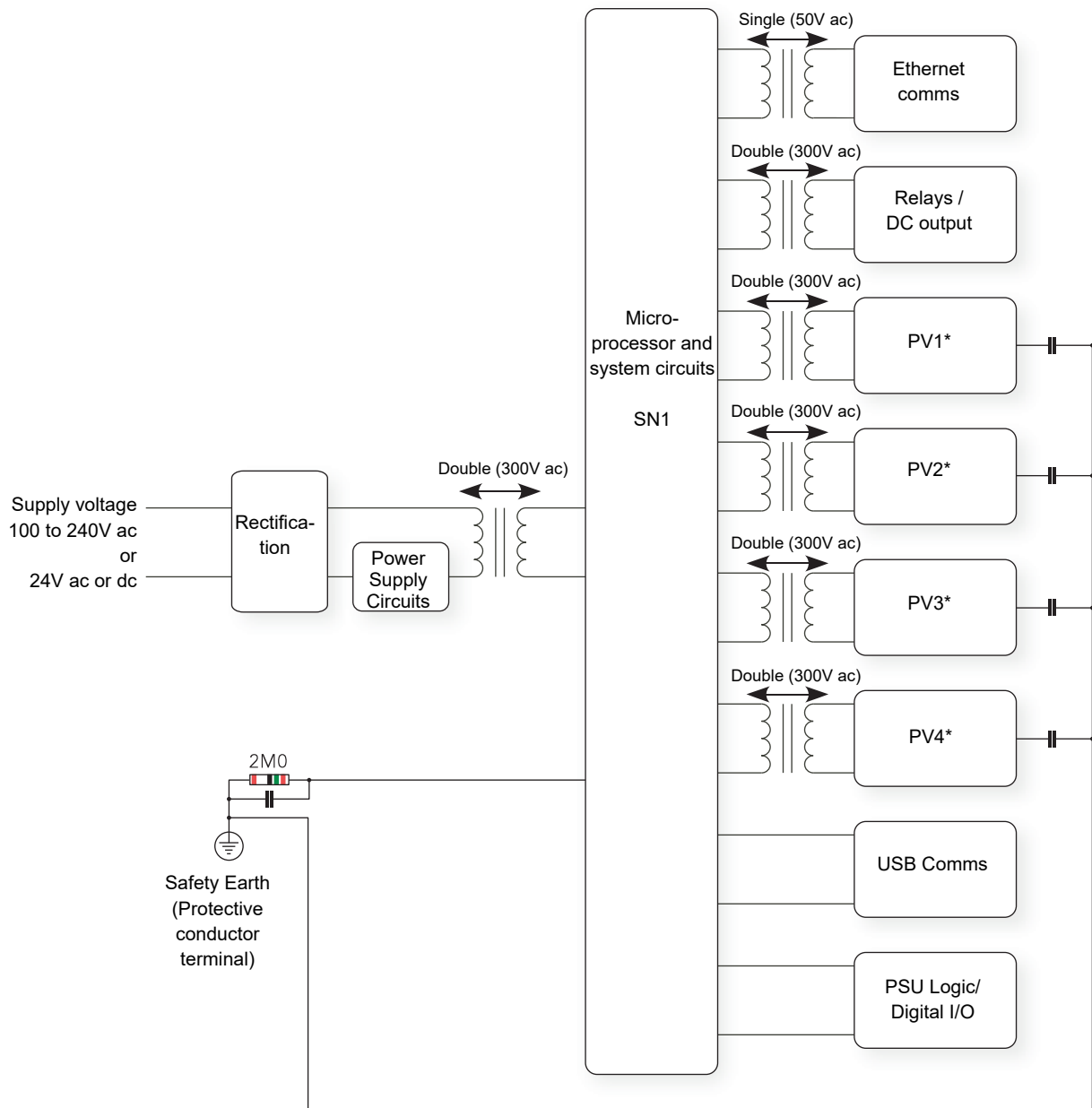
Figure 224 Isolation diagram
