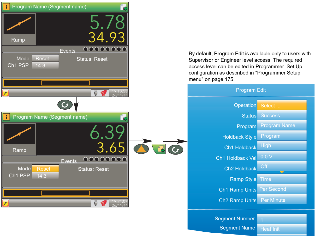
Figure 31 Access to the program editor
