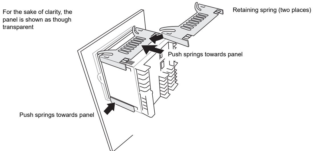
Figure 1 Securing the Instrument
