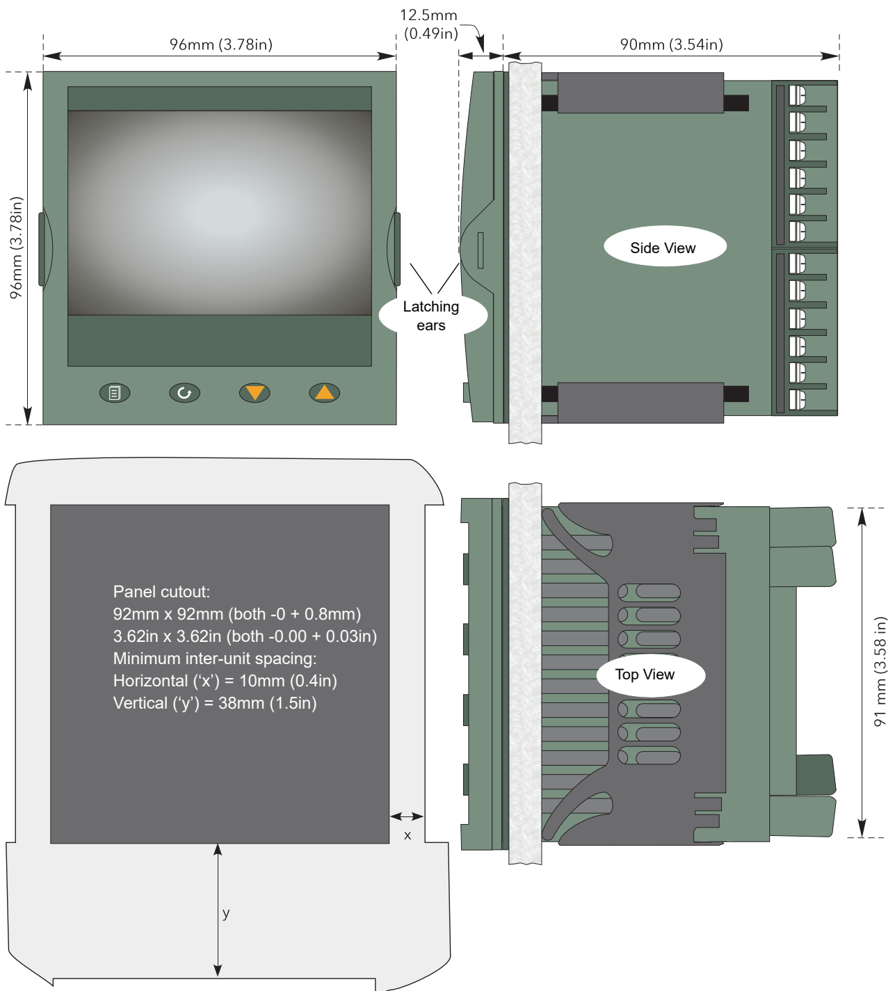
Figure 2 Mechanical installation details (standard case)
