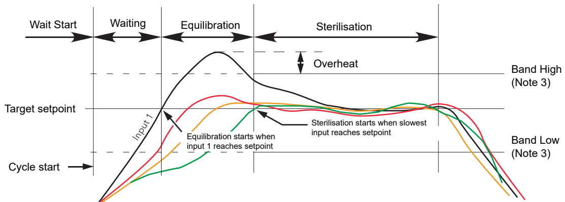
Figure 42 Steriliser cycle
