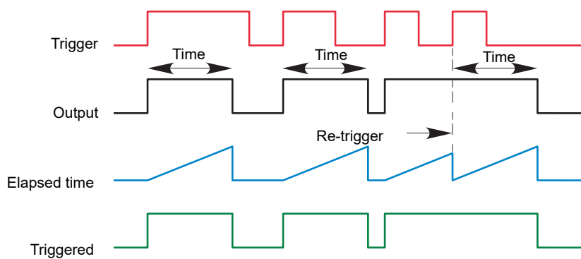
Figure 153 'On Pulse' definitions ON DELAY
