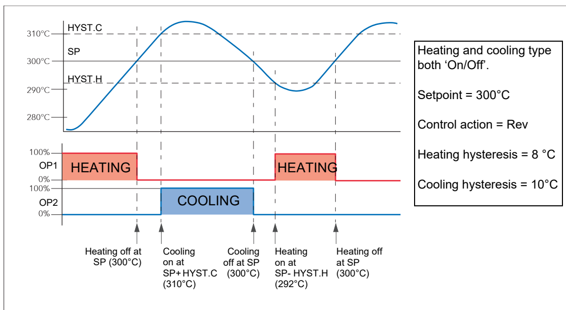
Figure 217 Deadband OFF
