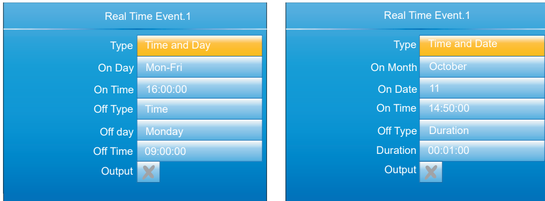
Figure 159 Real Time Events (typical)
