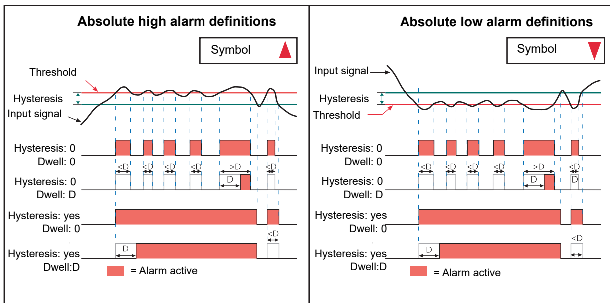
Figure 94 Absolute alarm parameters
