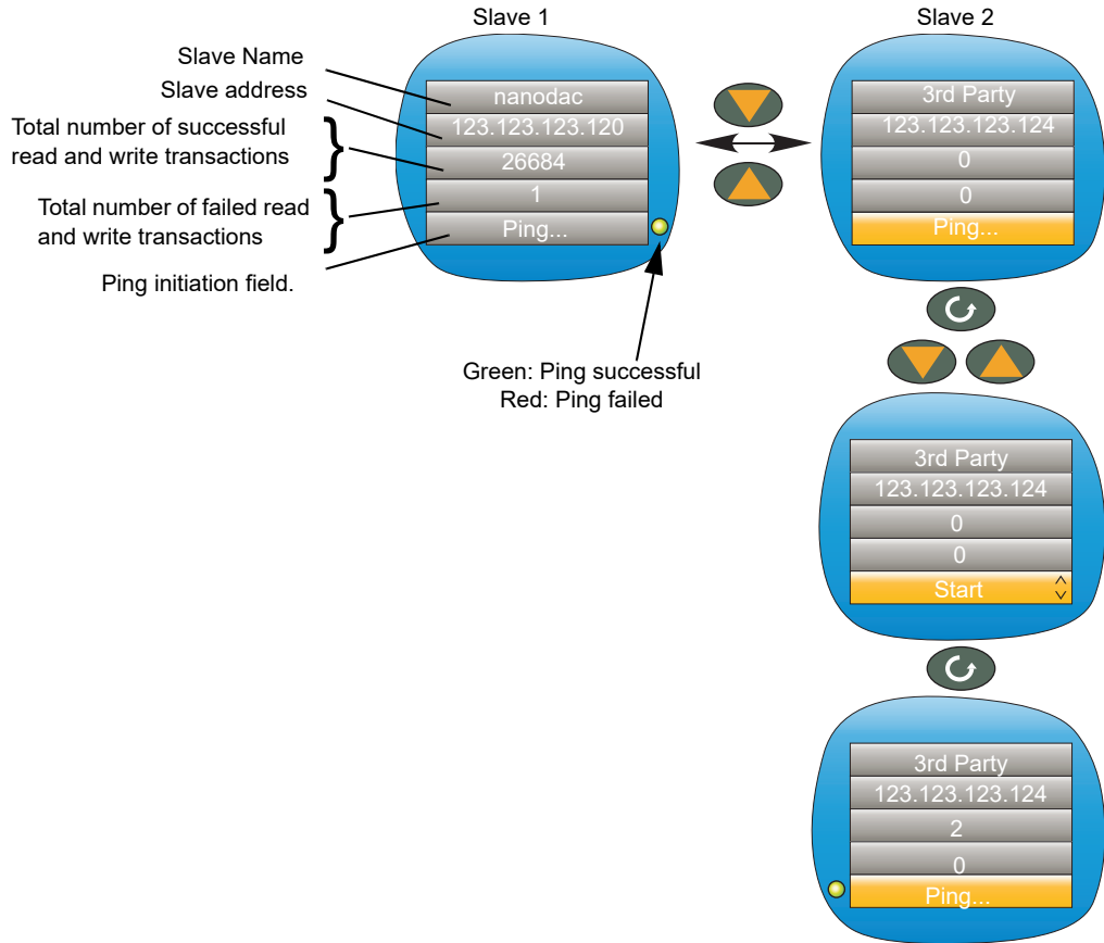
Figure 48 Slave 2 ping initiation (Slave 1 similar)
