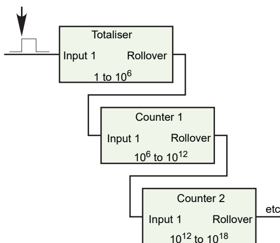
Figure 101 Cascading counters
