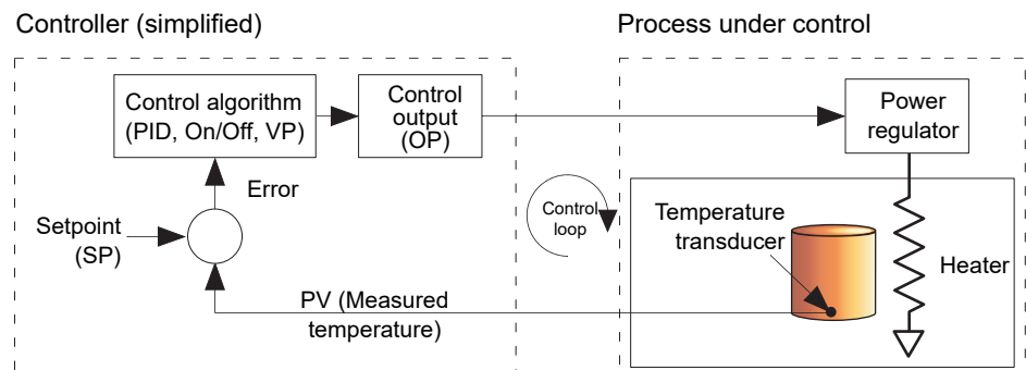
Figure 198 Control loop example
