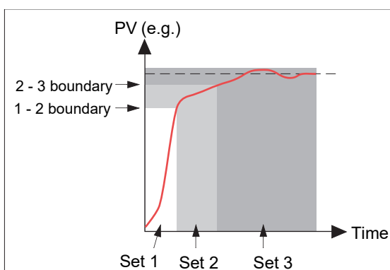
Figure 204 Gain scheduling
