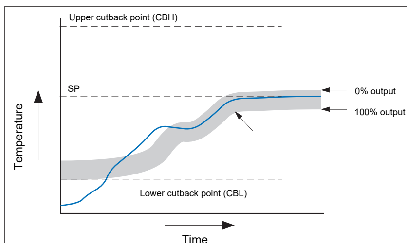
Figure 203 Cutback operation
