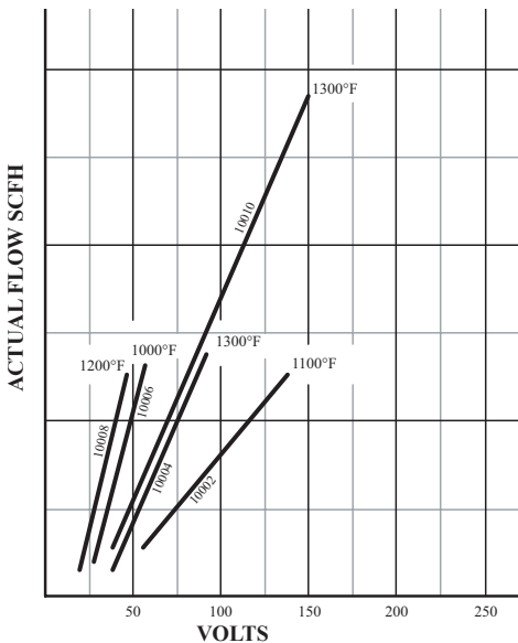
Nozzled Air Heaters
