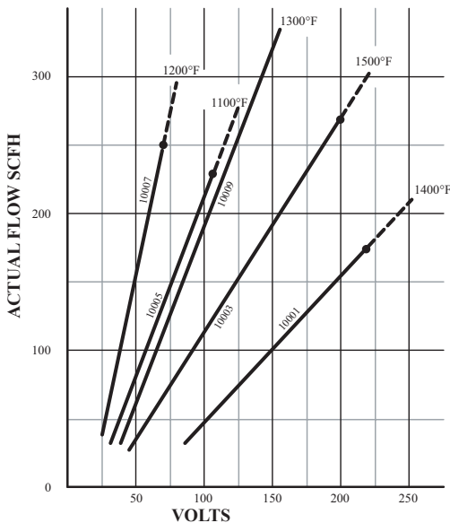
Open Air Heaters
