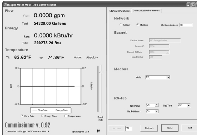
Figure 3: Communication Parameters
