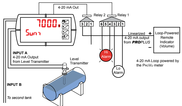
Round Horizontal Tank Signal Input Conditioning
