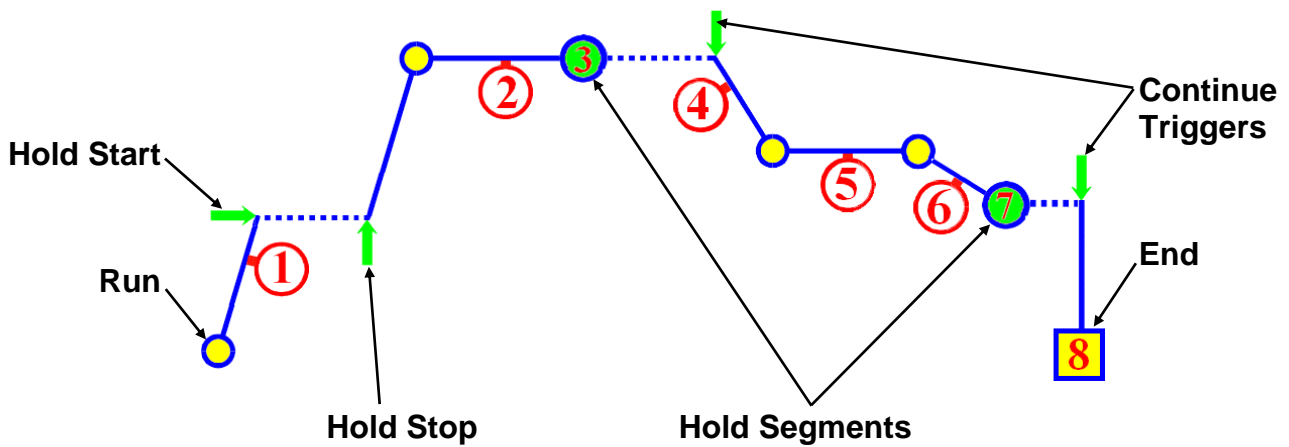
Figure 51. Run/Hold & Hold Segments
