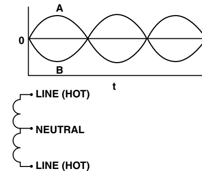
Figure 1. 1Ø System
