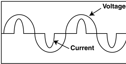
Figure 7 Nonlinear current draw
