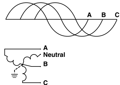
Figure 3. 3Ø, 4-Wire System
