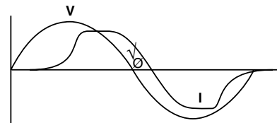
Figure 5. Power factor on nondistorted sine wave.
