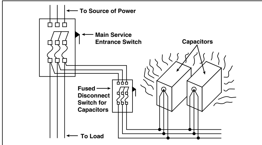
Figure 10. Power factor capacitors at resonant frequency.
