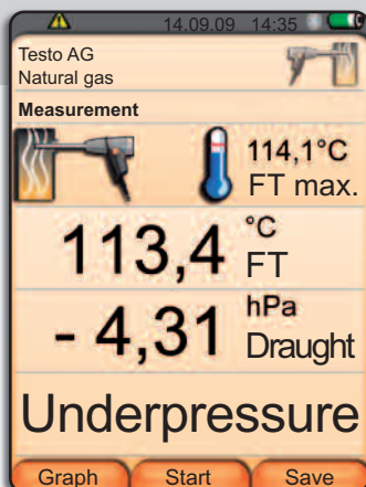
The result of the measurement: a negative pressure exists (-4.31 hPa)
