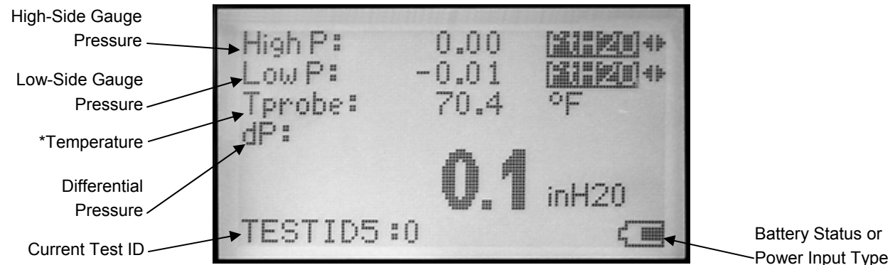
Figure 3: Pressure Measurement Screen
