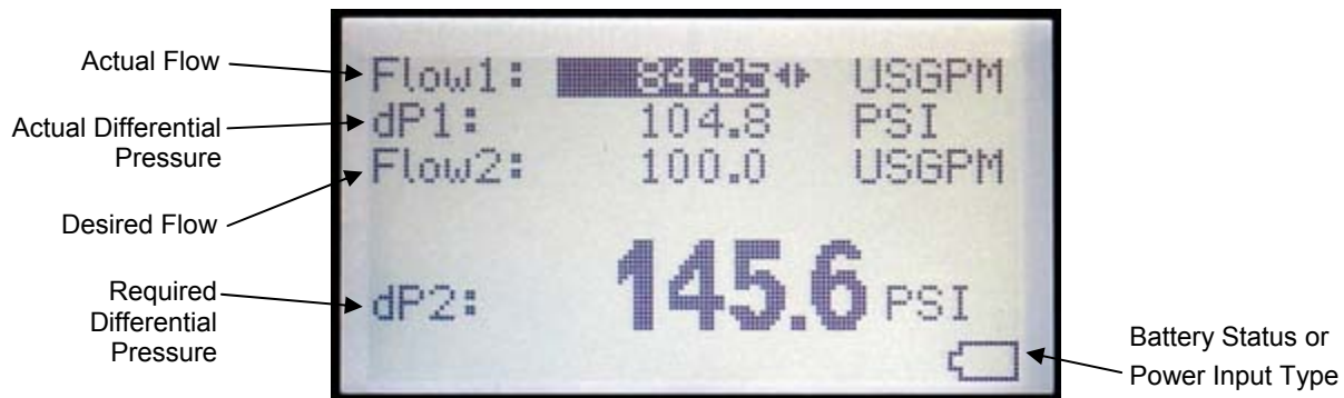
Figure 12: Pump Law Delta P Screen
