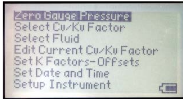
Figure 5: Main Menu
