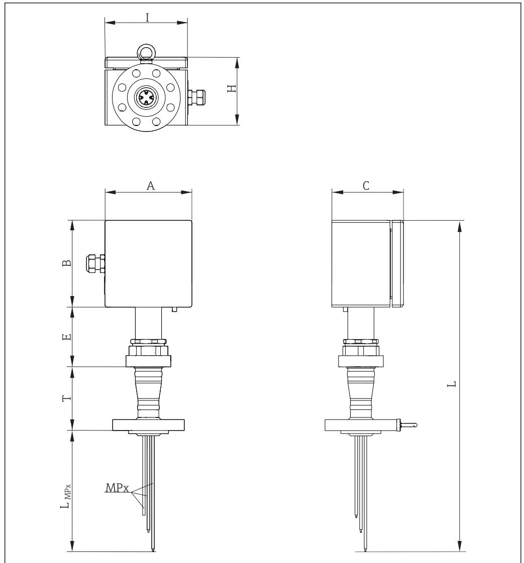
10 Design of the modular multipoint thermometer, with tube neck design. All dimensions in mm (in)
