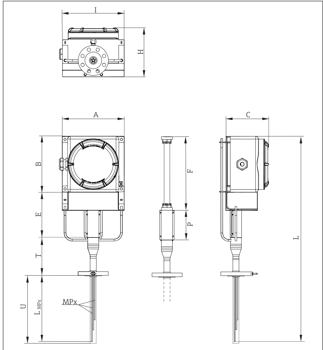
9 Design of the modular multipoint thermometer, with frame neck. All dimensions in mm (in)
