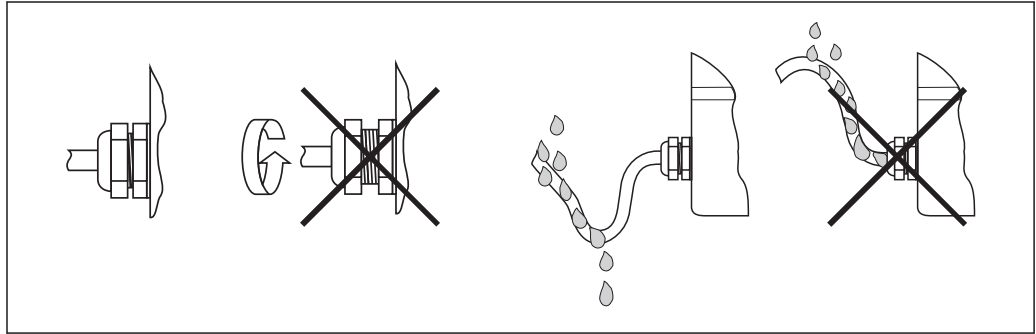
8 Connection hints to maintain IP protection
