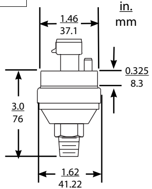
Figure 7 Dimensional Drawing
