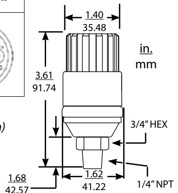
Figure 6 Dimensional Drawing
