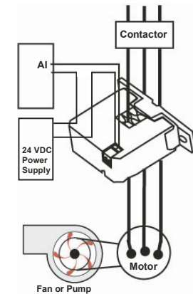
Figure 2: CTCG420NN
