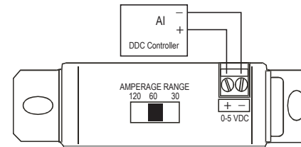
Figure 8: CTCGV05NN Wiring
