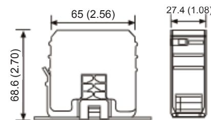
Figure 1: CSC Dimensions mm. (in.)
