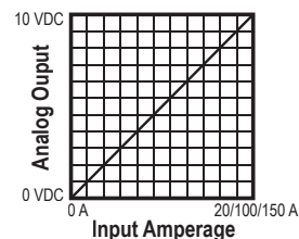
Figure 11: CTCGV10NN Linear Output
