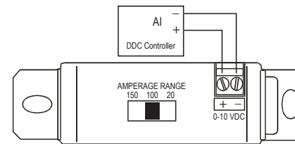
Figure 10: CTCGV10NN Wiring
