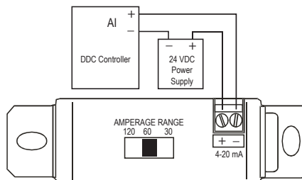
Figure 6: CTCG420NN Wiring
