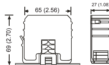
Figure 1: CSC Dimensions mm. (in.)
