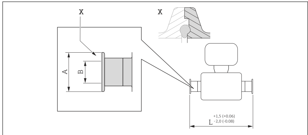
36 Detail X: Asymmetrical process connection; the part shown in gray is provided by the supplier. Engineering unit mm (in).
