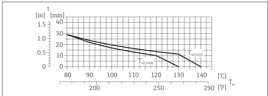
31 Maximum recommended insulation thickness depending on the temperature of the medium and the ambient temperature
