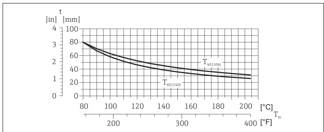
32 Maximum recommended insulation thickness depending on the temperature of the medium and the ambient temperature
