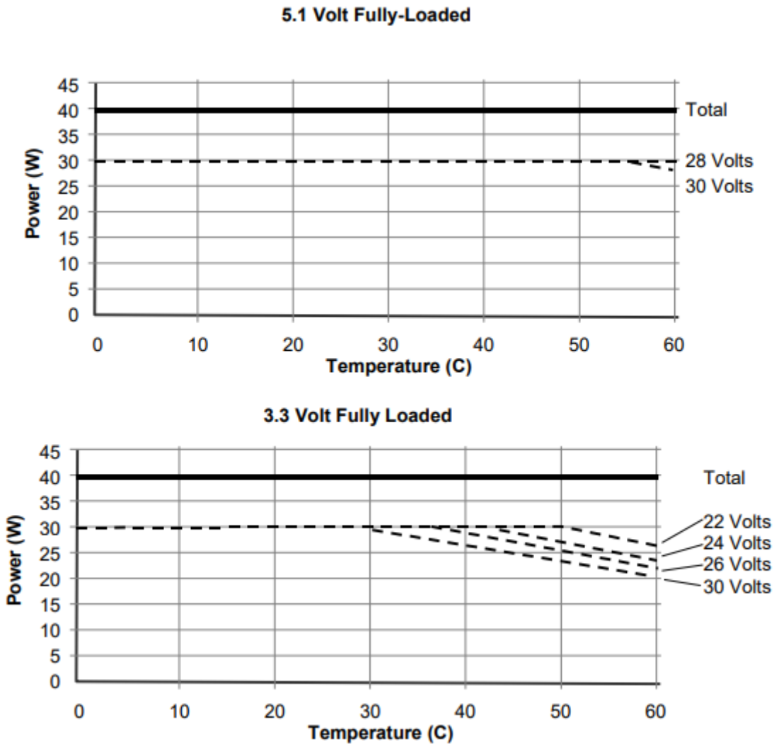
Figure 3: Thermal Derating
