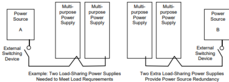
Figure 9: Powersupply Redundancy
