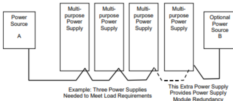
Figure 8: Powersupply Redundancy
