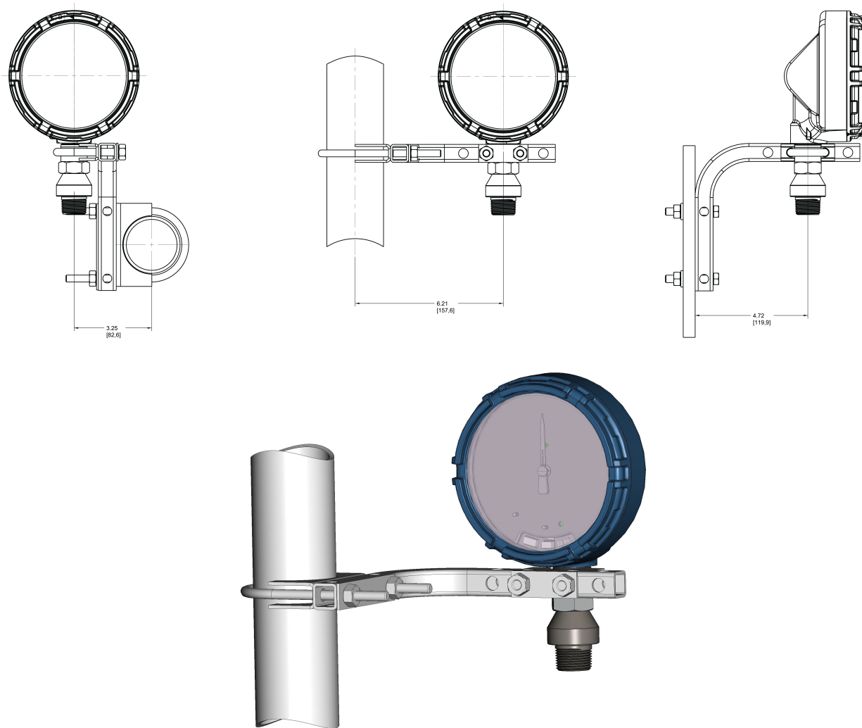
Figure 6: Mounting Configurations (B4 bracket)
