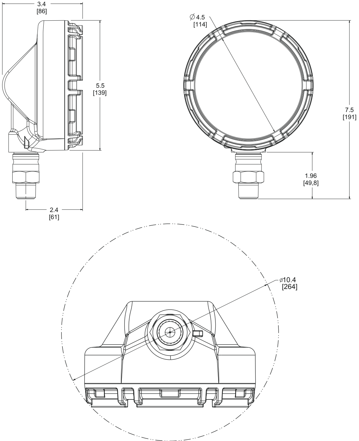
Figure 2: Rosemount Wireless Pressure Gauge with 1/2-14 NPT Male or G1/2 Male Process Connection
