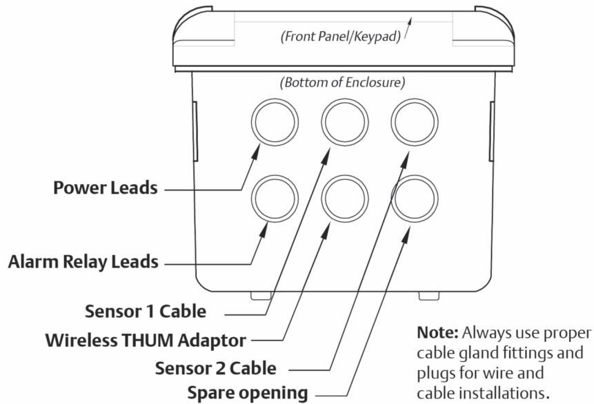
Figure 3-5 56 Recommended Wire Entry and THUM Adaptor Installation
