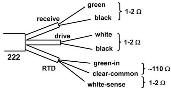
FIGURE 13. Disconnect wires from analyzer before measuring resistance.
