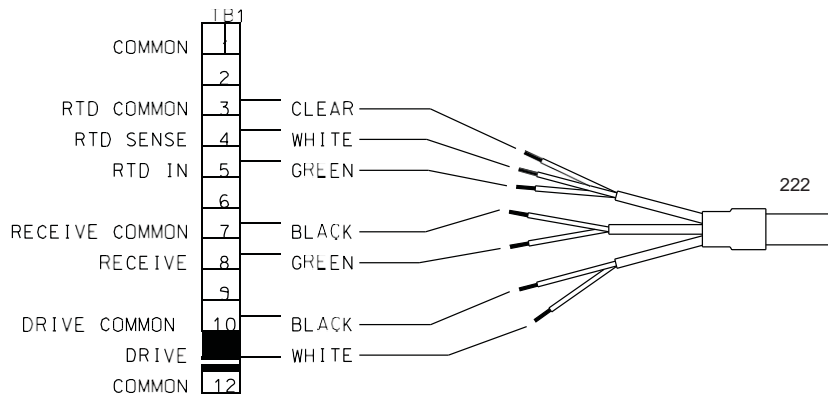
FIGURE 6. Wiring 222 sensor to 54eC analyzer
