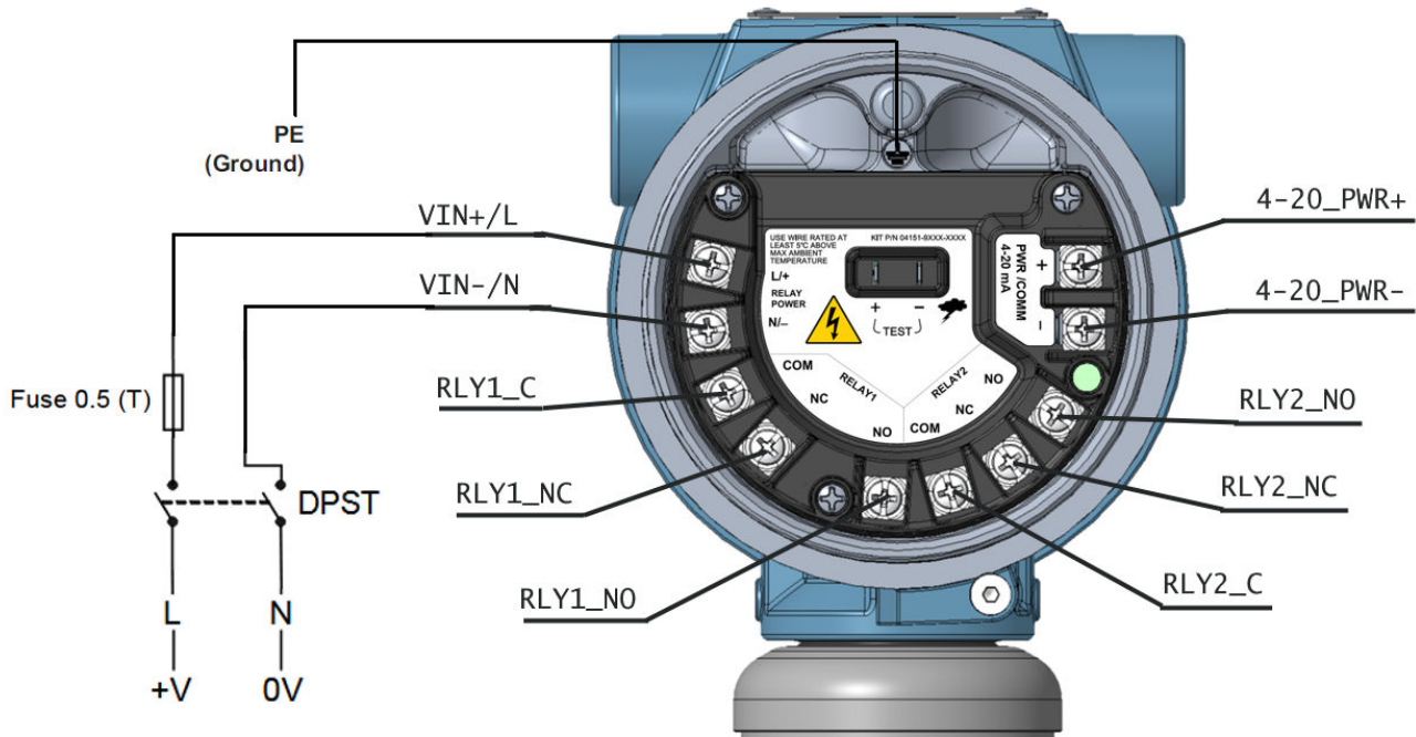
Figure 1: Relay Switches
