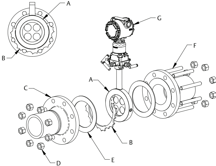
Figure 10. Rosemount 405 Installation
