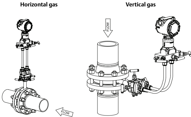
Figure 5. Remote Mount
