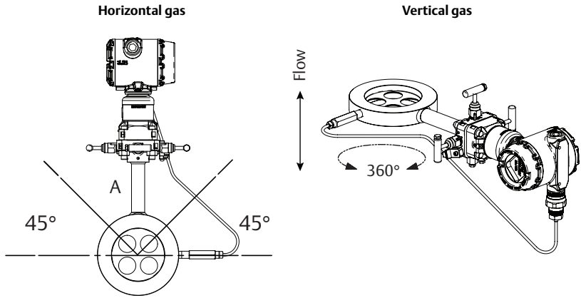
Figure 4. Direct Mount
