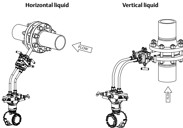
Figure 3. Remote Mount
