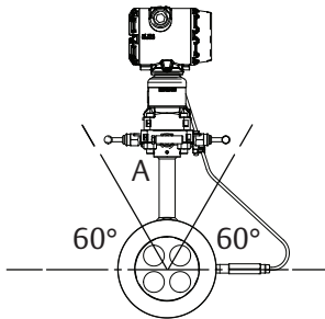
Figure 8. Direct mount — 405C, 405P, and 405A
