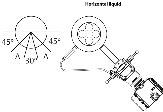
Figure 2. Direct Mount
