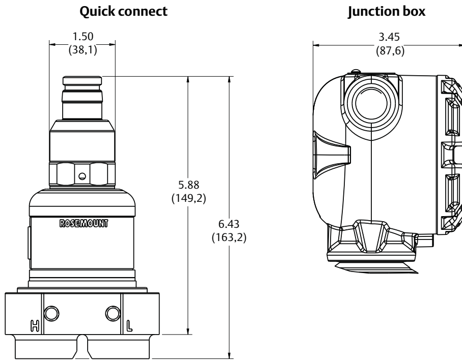
Figure 3. Other Housings
