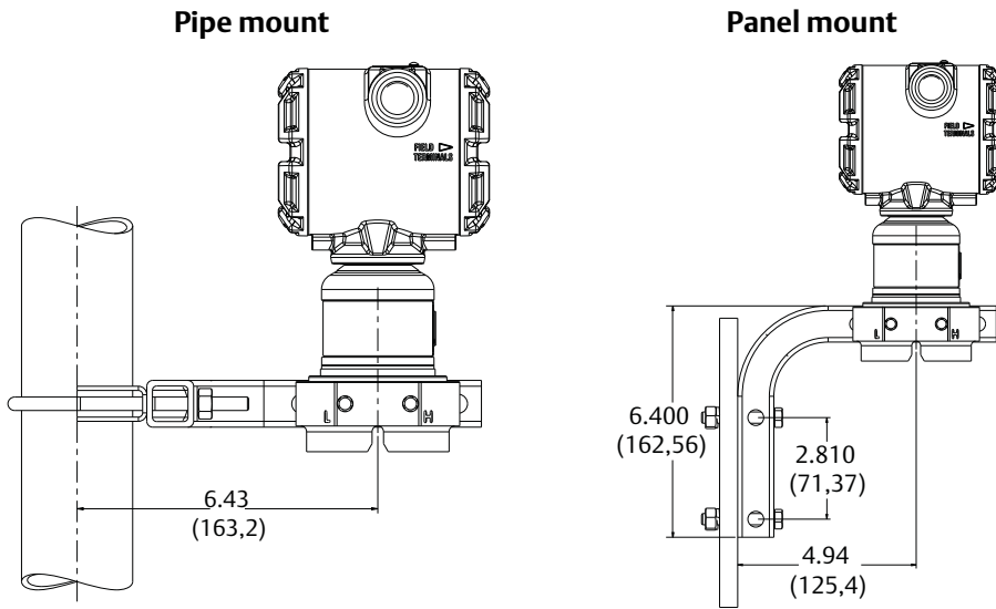
Figure 6. Traditional Mounting Configurations
