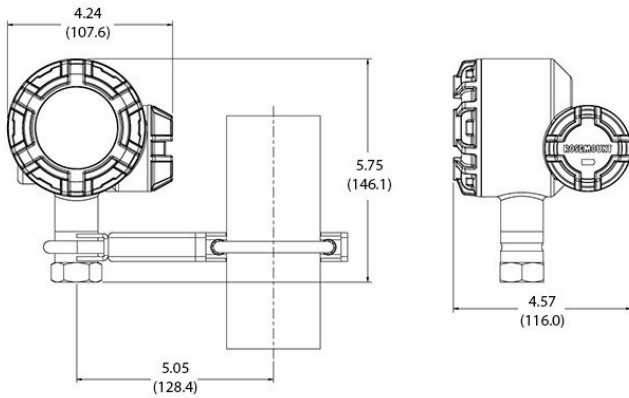
Figure 3-4: Remote Mount
