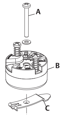
Figure 1. Rosemount 148 Transmitter Accessories
