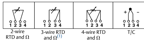
Figure 2. 148 Sensor Connections Diagram
