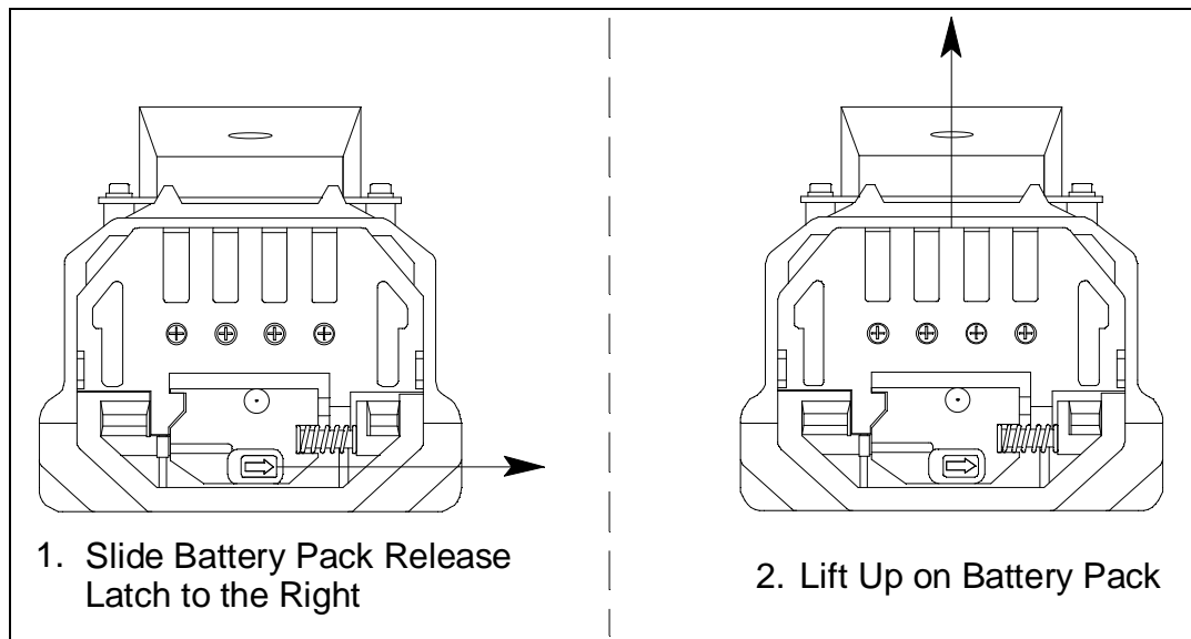
Figure 14: Releasing the Battery Pack
