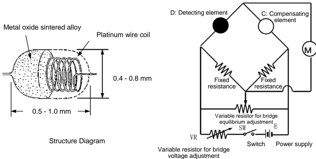
Basic Circuit
