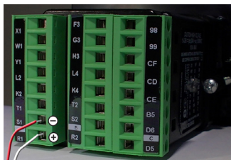
Figure 2: Input Terminal Connection Shown Here
