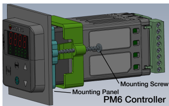
Figure 1: PM6 Installation
