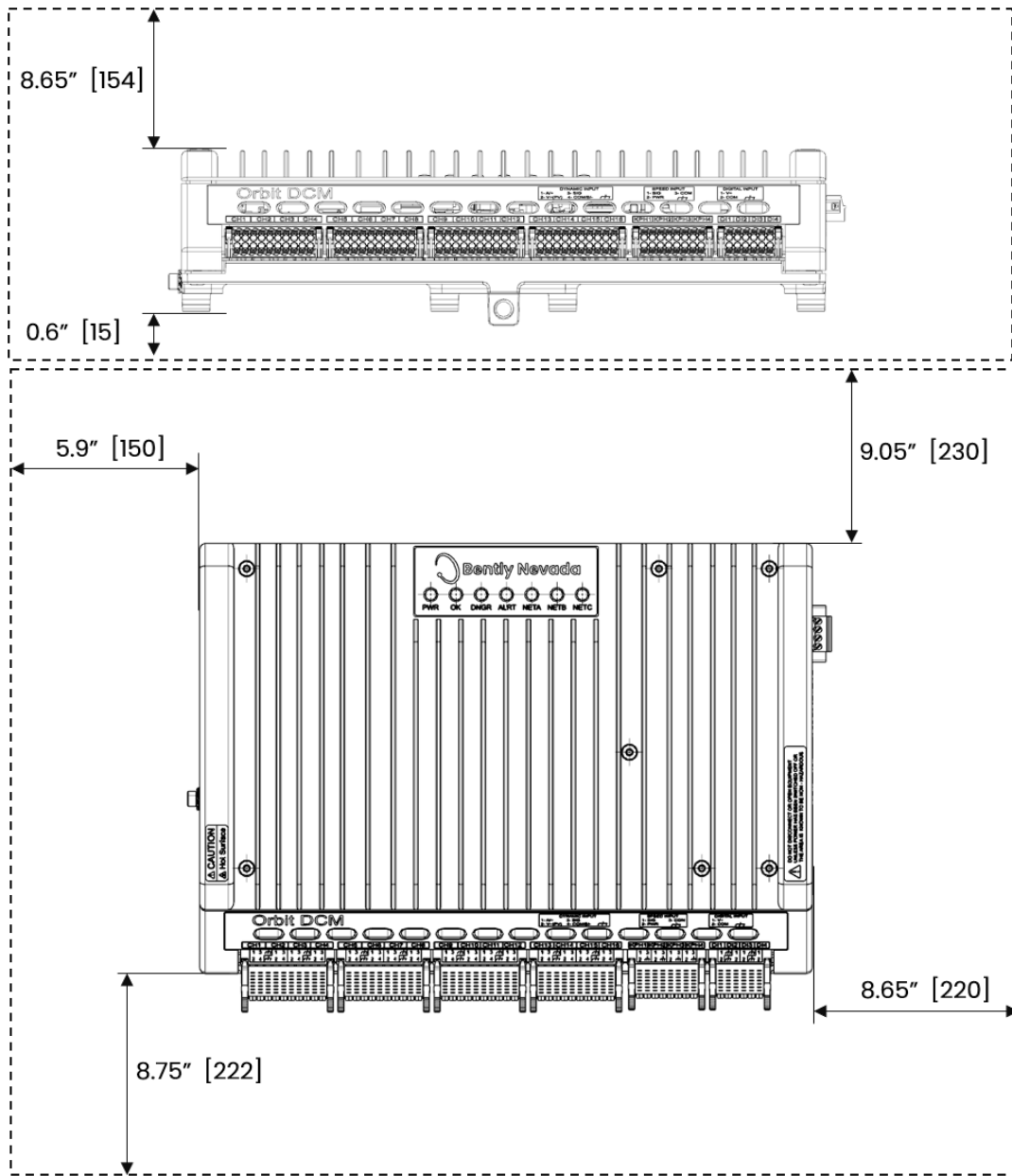
Figure 3: Minimum Housing Clearance
