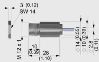
Sensing head (standard)
