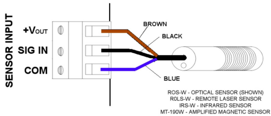
Sensor Connection Detail
