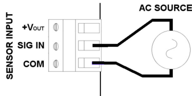
Sensor Connection Detail
