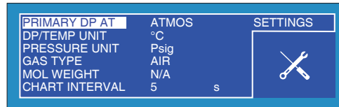
Figure 15 SETTINGS Page
