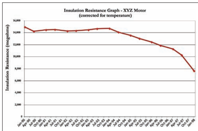
Figure 24: Insulation Resistance Graph Corrected for Temperature
