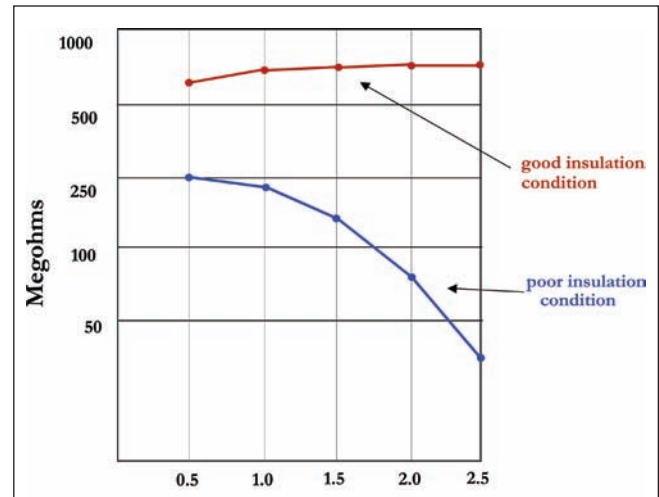
Figure 19: Step Voltage Step Graph
