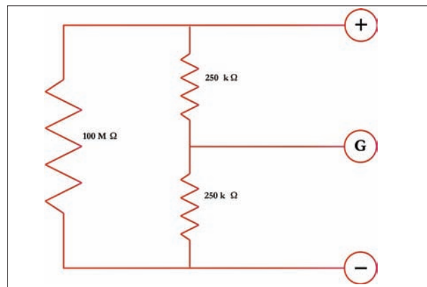
Figure 12: Guard Terminal Diagram
