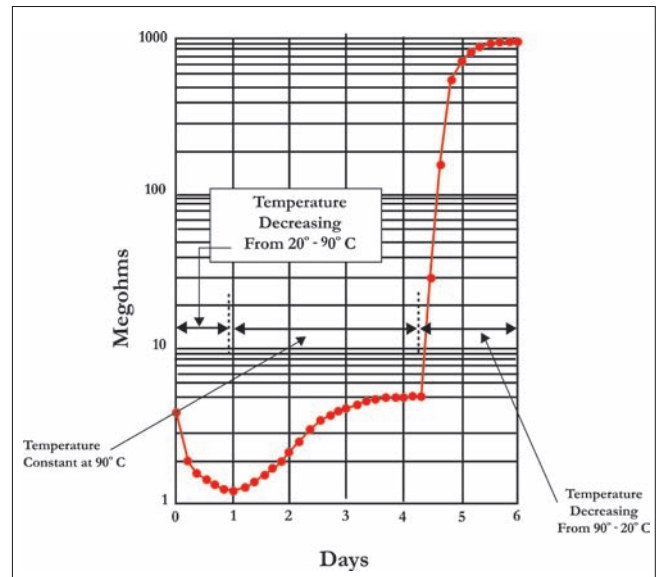
Figure 25: Typical Drying-out Resistance Graph
