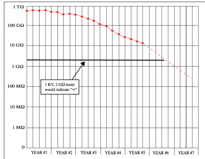
Figure 15: Changes in Insulation Resistance at High Values
