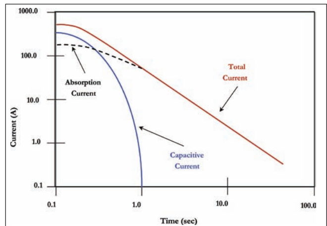
Figure 21: Reabsorption Currents
