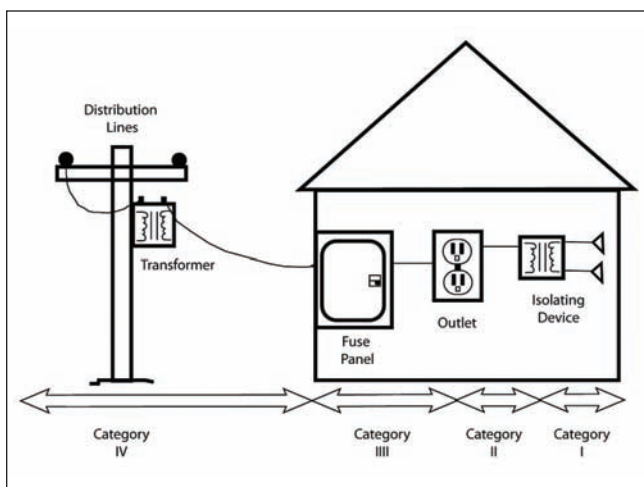
Figure 22: Electrical supply broken down into categories
