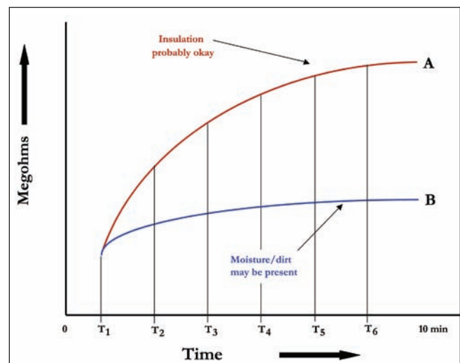
Figure 17: Time Resistance Test Graph
