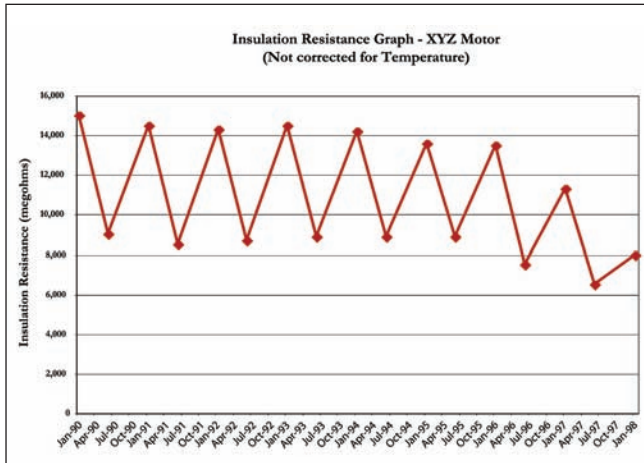
Figure 23: Insulation Resistance Graph Not Corrected for Temperature
