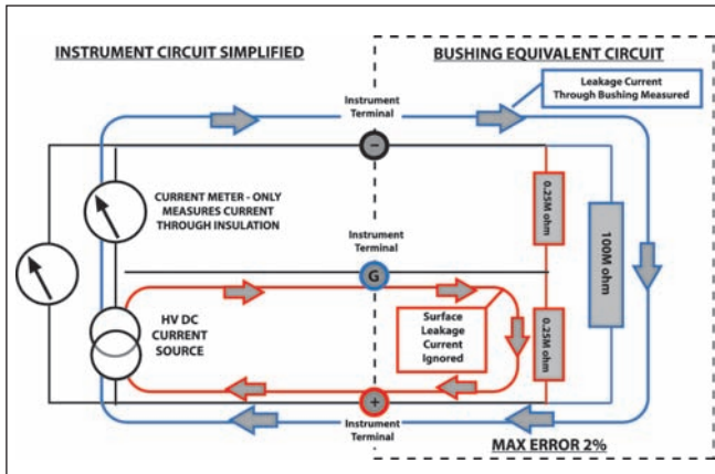
Figure 14: Instrument circuit simplified
