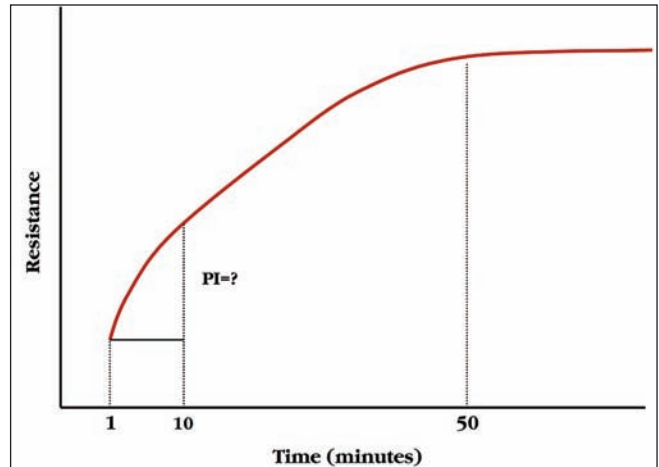
Figure 18: Benefit of the Polarization Test for Large Equipment
