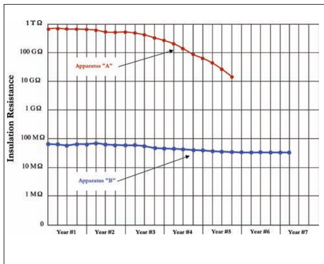
Figure 16: Comparison of Trended Test Results
