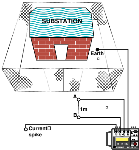
Determining 'Step' potential
