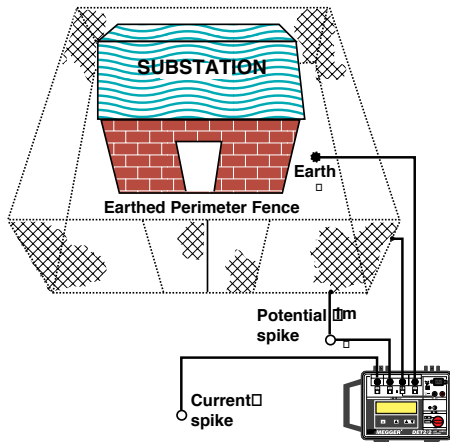
Determining 'Touch' potential.
