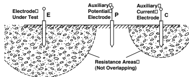
Resistance areas associated with an earth electrode and current spike.
