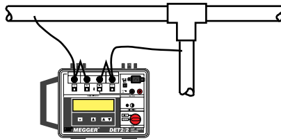
Continuity testing.
