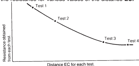
Example of possible results from several Slope method tests.
