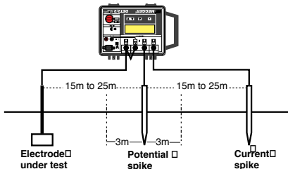
Fall-of-Potential method using a single lead to the earth electrode.
