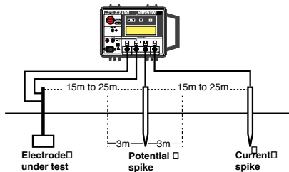
Fall-of-Potential method connections.
