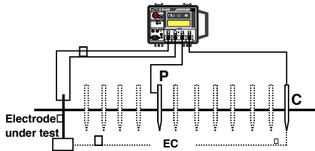
Connections for the Slope method
