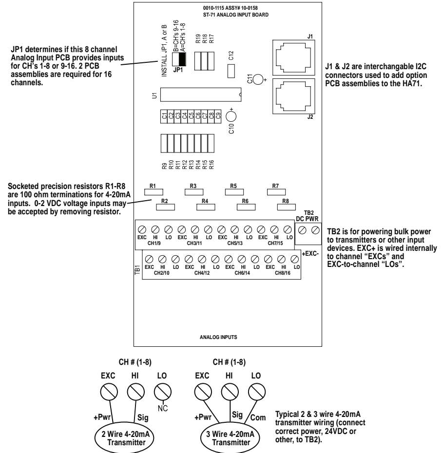
Figure 3-3. 8 Channel Analog Input Option 10-0158
