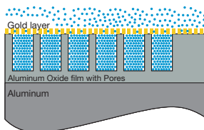
Operating Principle of Al_2O_3 Sensor
