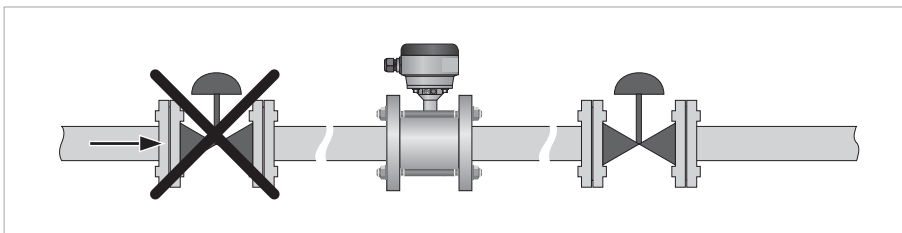
Figure 2-11: Installation in front of a control valve
