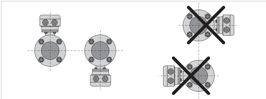
Figure 2-14: Mounting position
