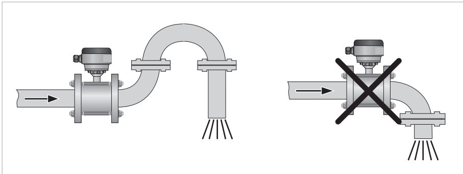
Figure 2-8: Installation in front of an open discharge
