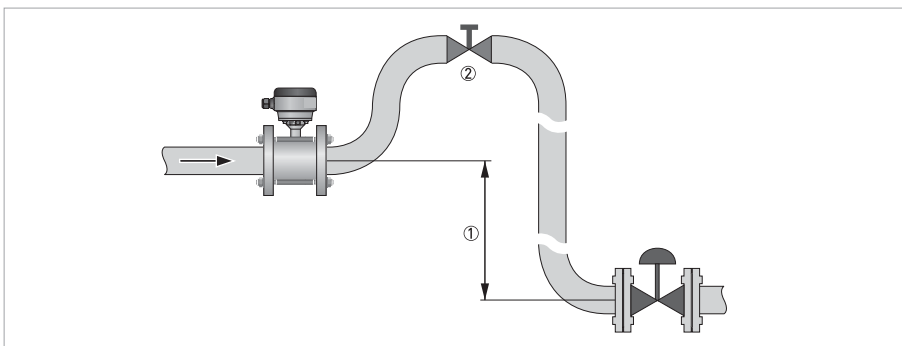
Figure 2-12: Air venting
