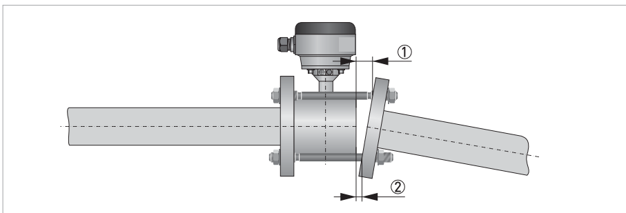
Figure 2-9: Flange deviation
