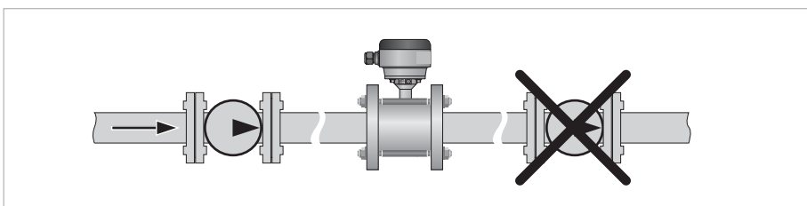
Figure 2-10: Installation behind a pump
