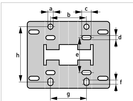
Figure 2-3: Dimensions of mounting plate of wall-mounted housing
