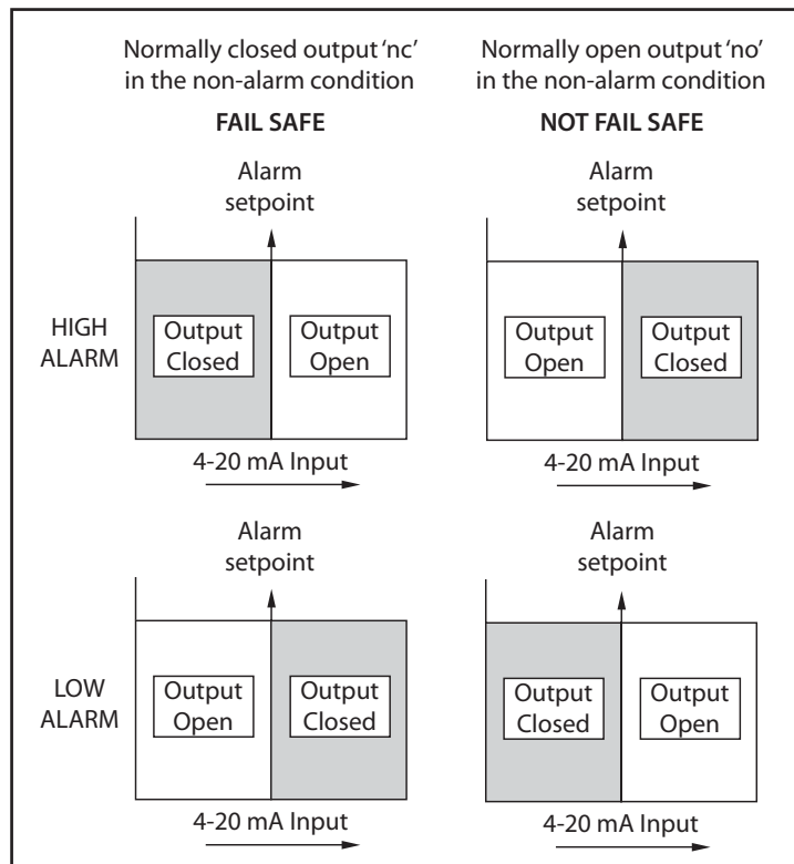
Figure 8 Alarm Outputs
