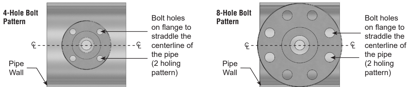
Figure 5. Flange Orientation
