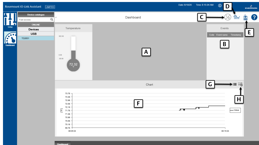
Figure 4-1: Dashboard Components
