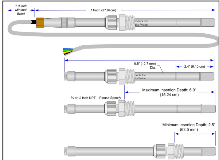
The HP125 Series Smart Probe
