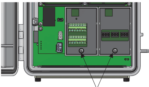
Tighten the screw on installed modules
