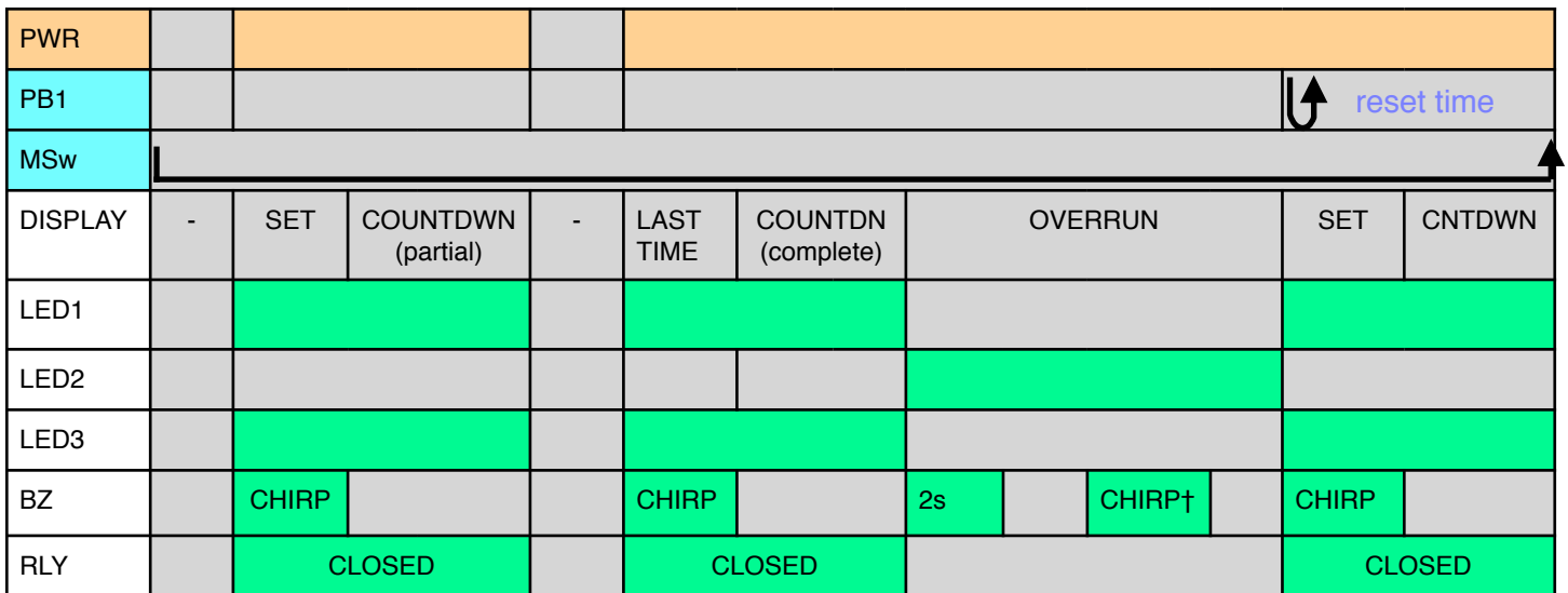
CHART 9.2 - Machine runtime - intermittent power
