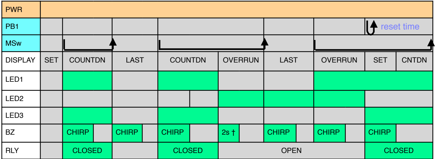
CHART 9.1 - Machine runtime.
