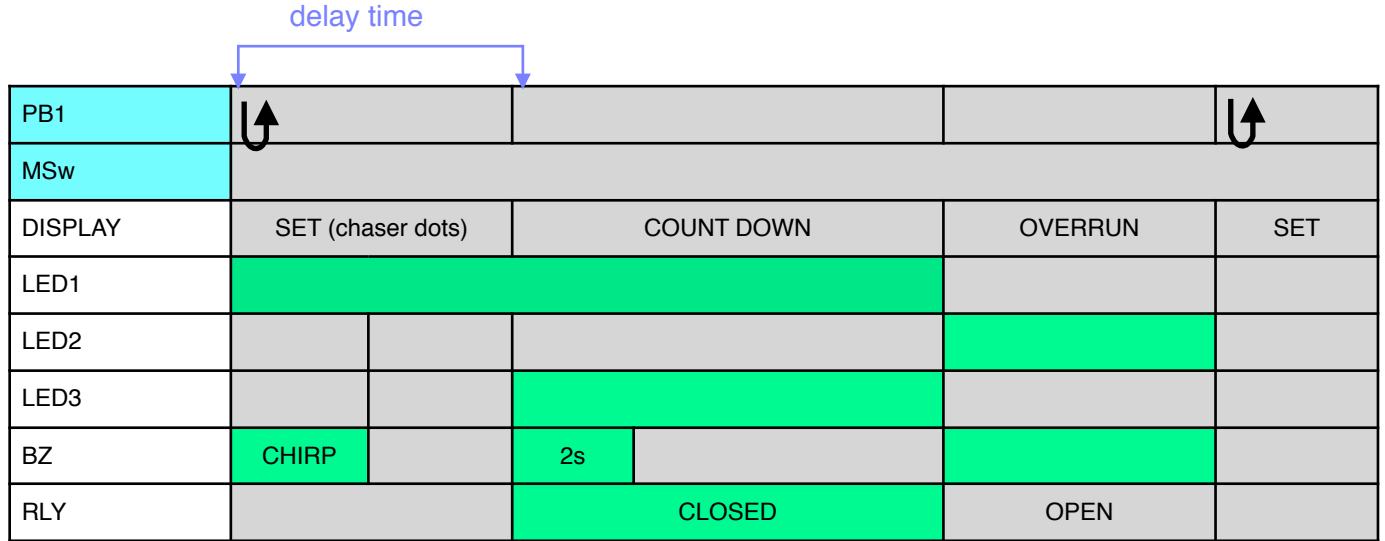
CHART 10.1 - CYCLE 10 COMPLETE CYCLE
