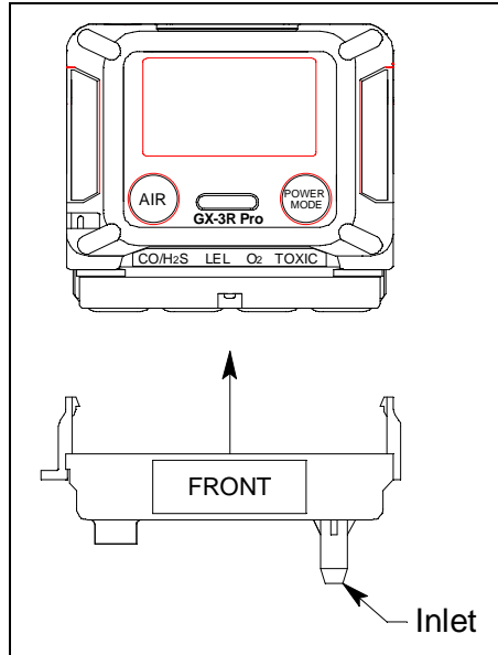
Figure 7: Calibration Cup Installation
