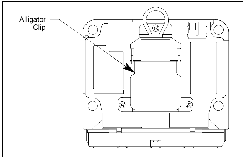
Figure 2: Alligator Clip
