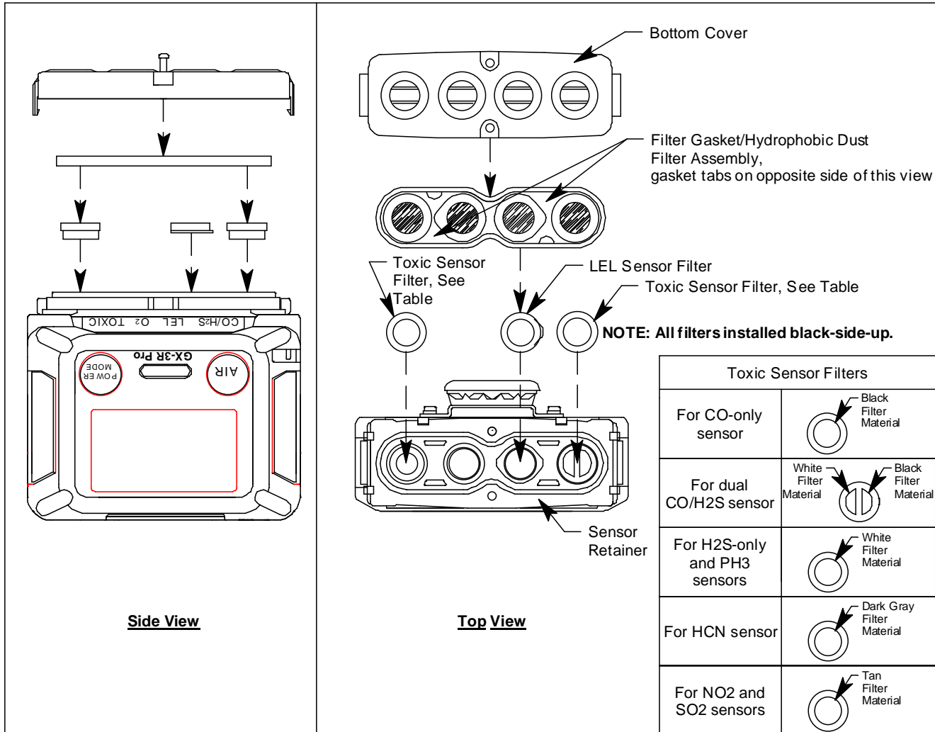
Figure 16: Replacing the Sensor Filters
