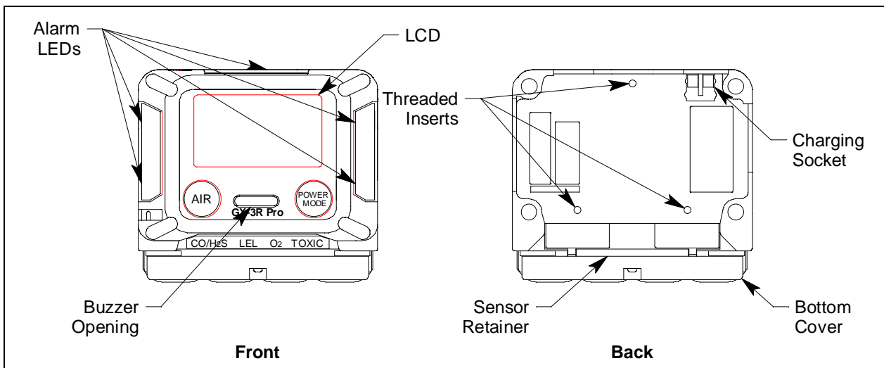
Figure 1: Component Location
