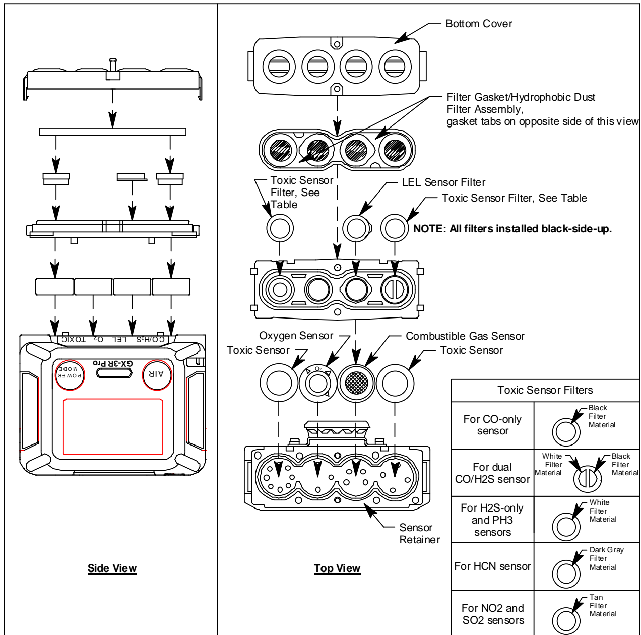
Figure 18: Replacing a Sensor
