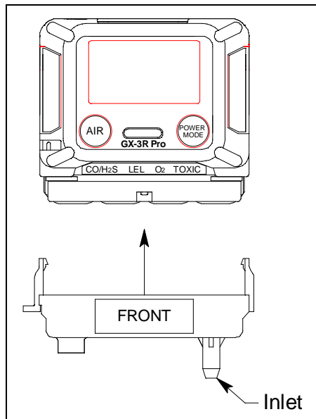
Figure 9: Calibration Cup Installation
