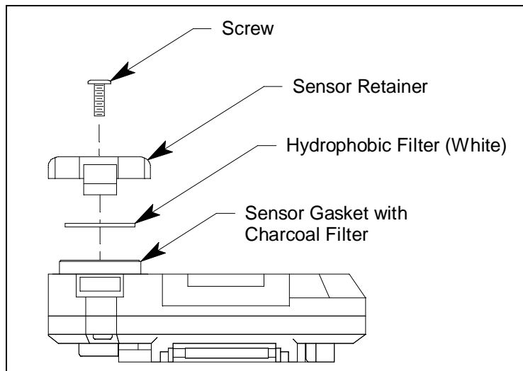
Figure 10: Replacing the Hydrophobic Filter
